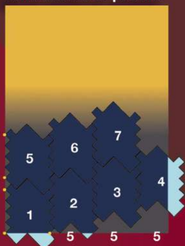
M044 Adoquín a soga
